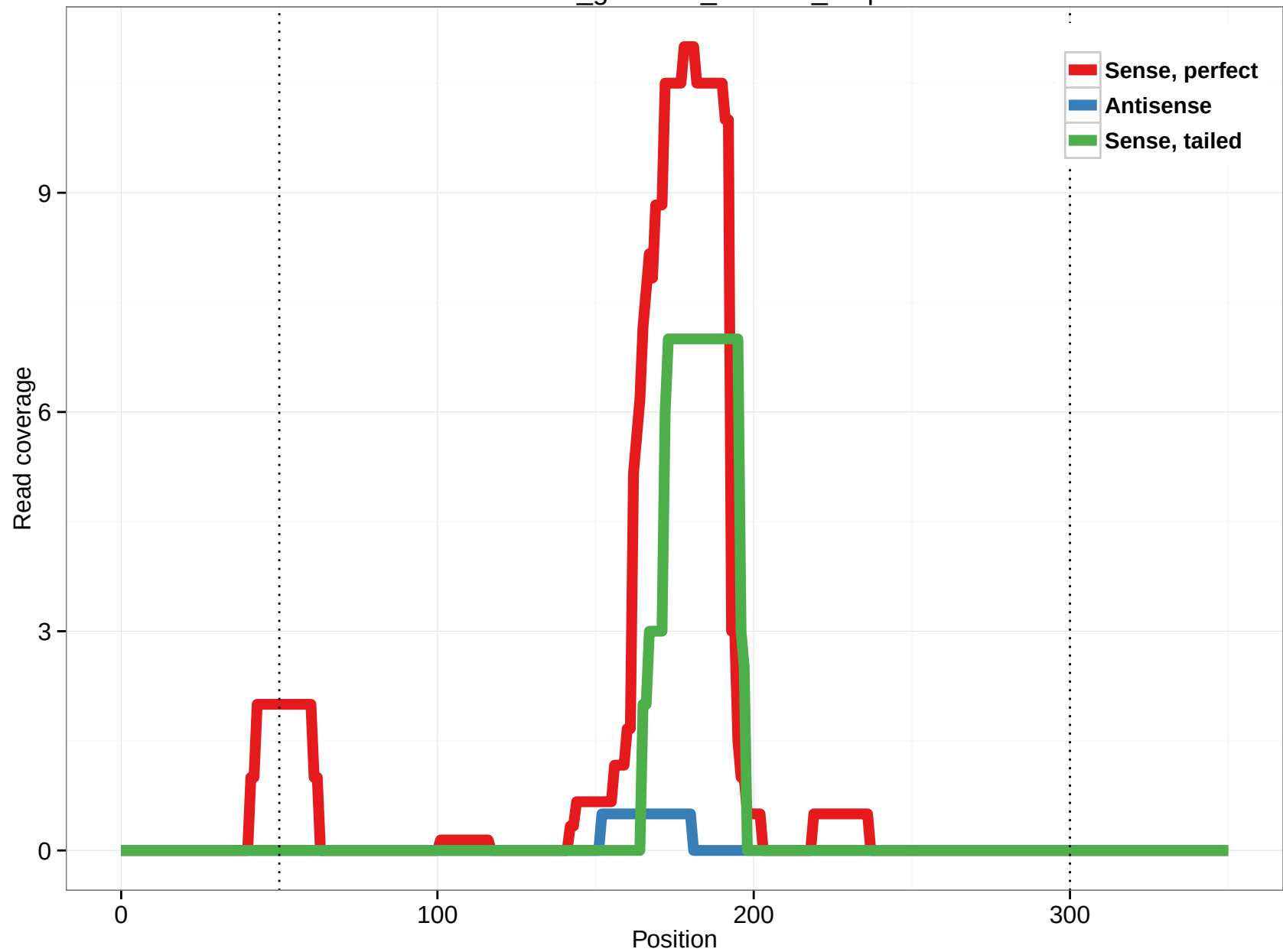
rheMac3_genscan_chr6.28_0.5p
