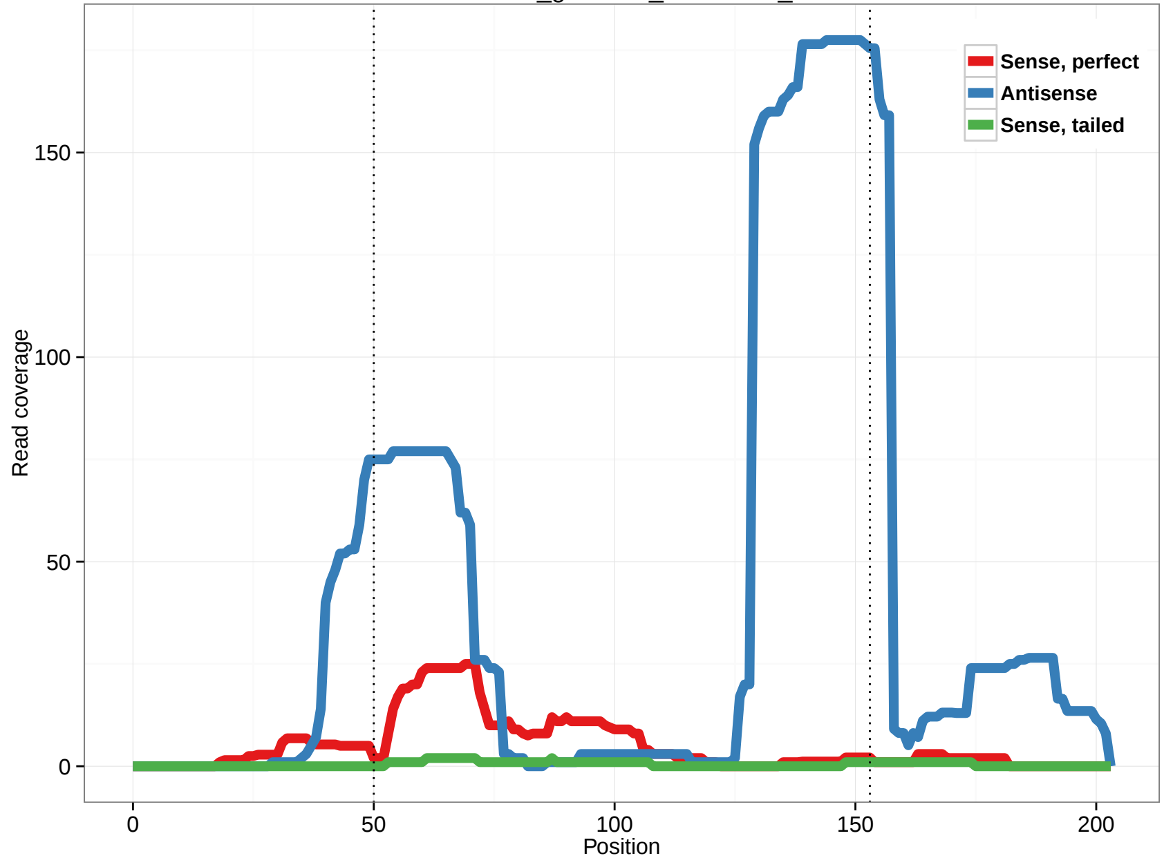
rheMac3_genscan_chr6.2787_1
