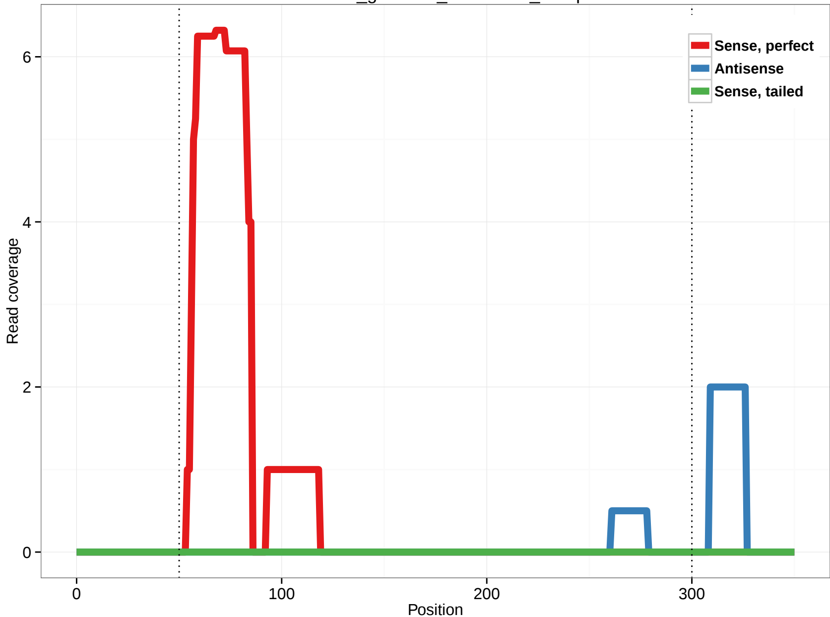
rheMac3_genscan_chr6.2681_21.5p
