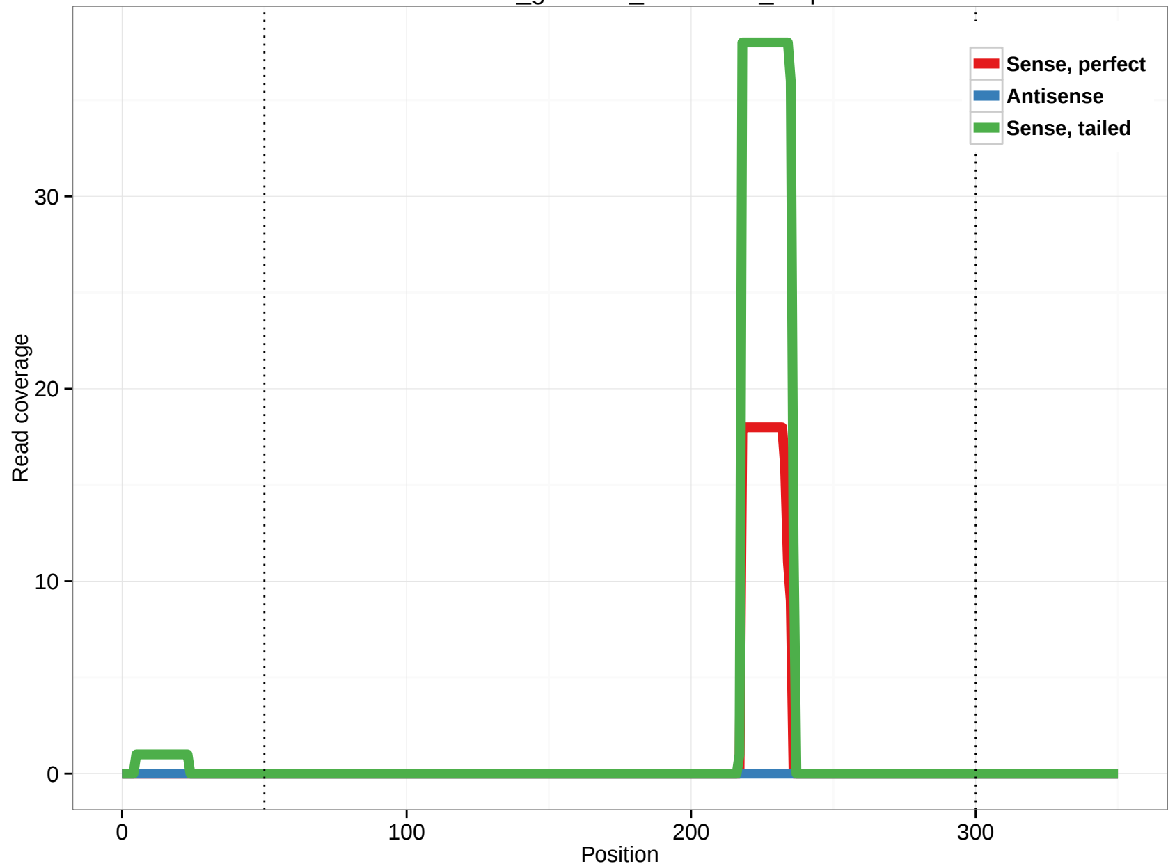
rheMac3_genscan_chr6.2649_3.5p
