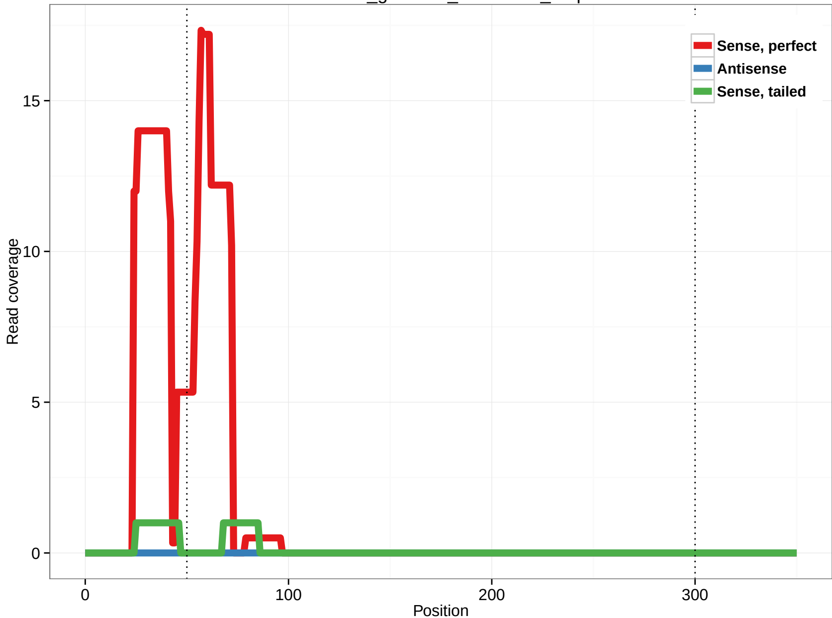
rheMac3_genscan_chr6.2628_1.5p
