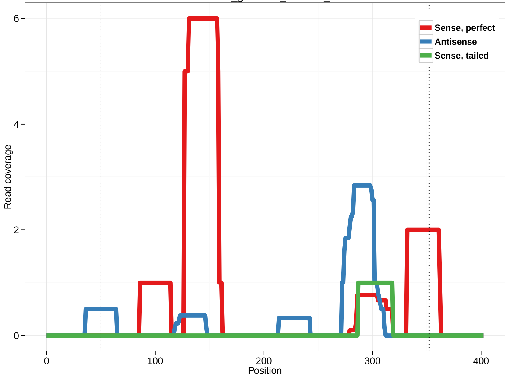
rheMac3_genscan_chr6.25_10
