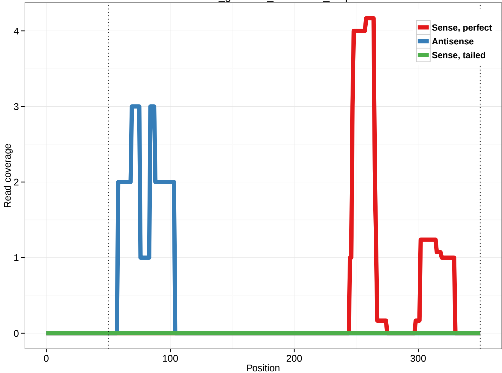
rheMac3_genscan_chr6.2412_0.5p
