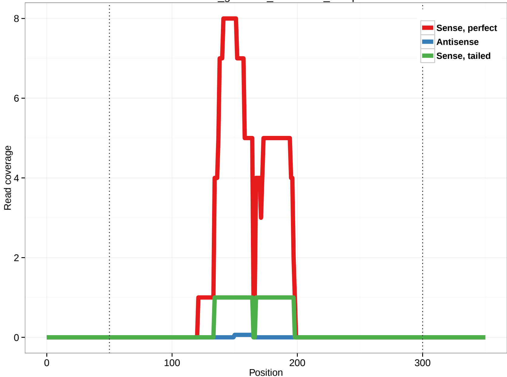
rheMac3_genscan_chr6.2353_10.5p
