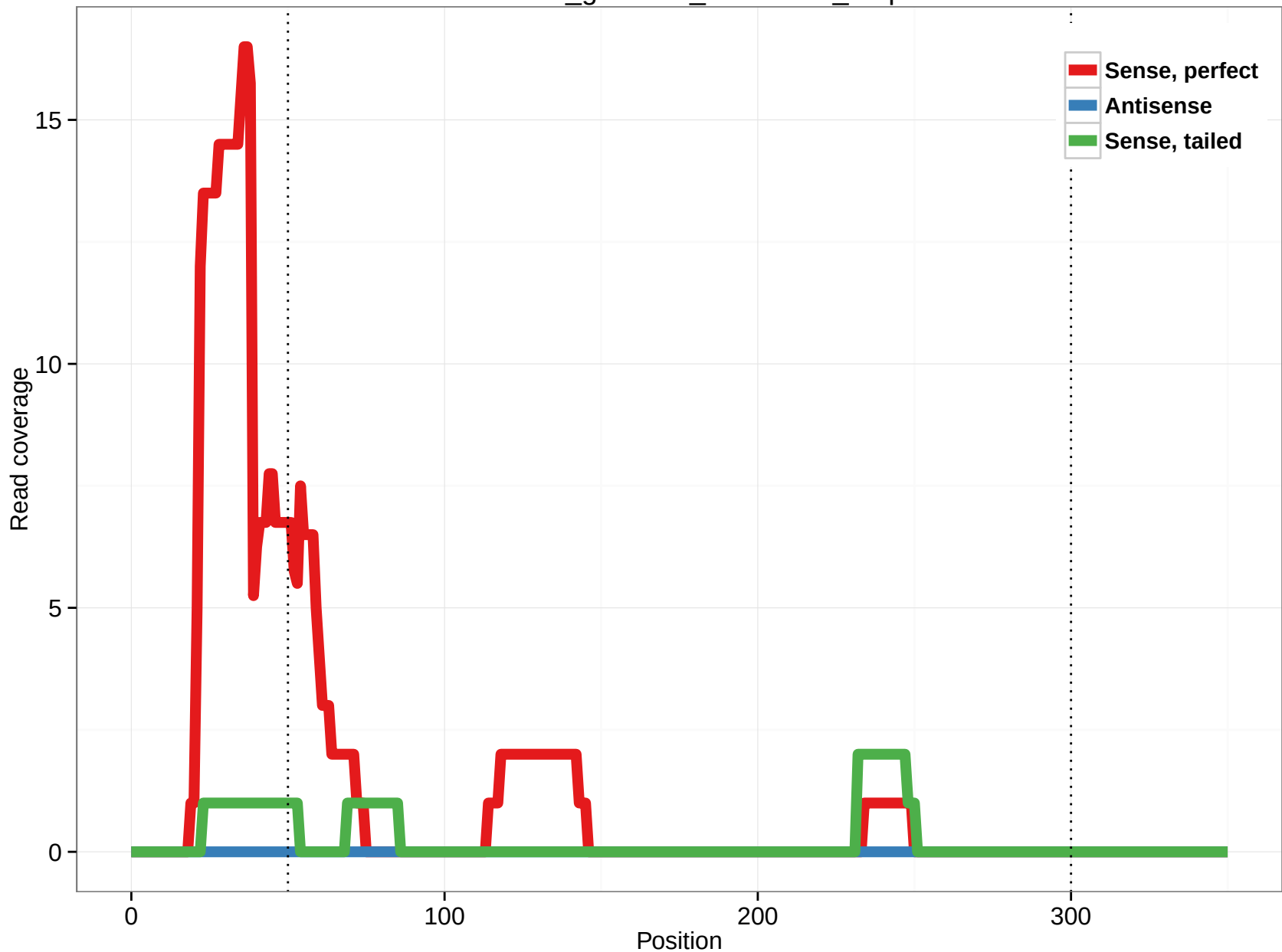
rheMac3_genscan_chr6.2350_0.5p
