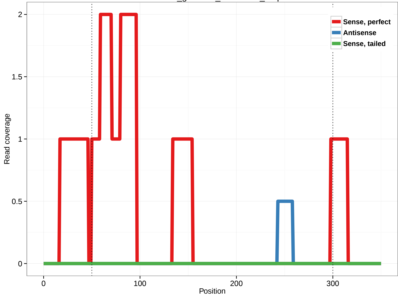
rheMac3_genscan_chr6.2349_1.5p
