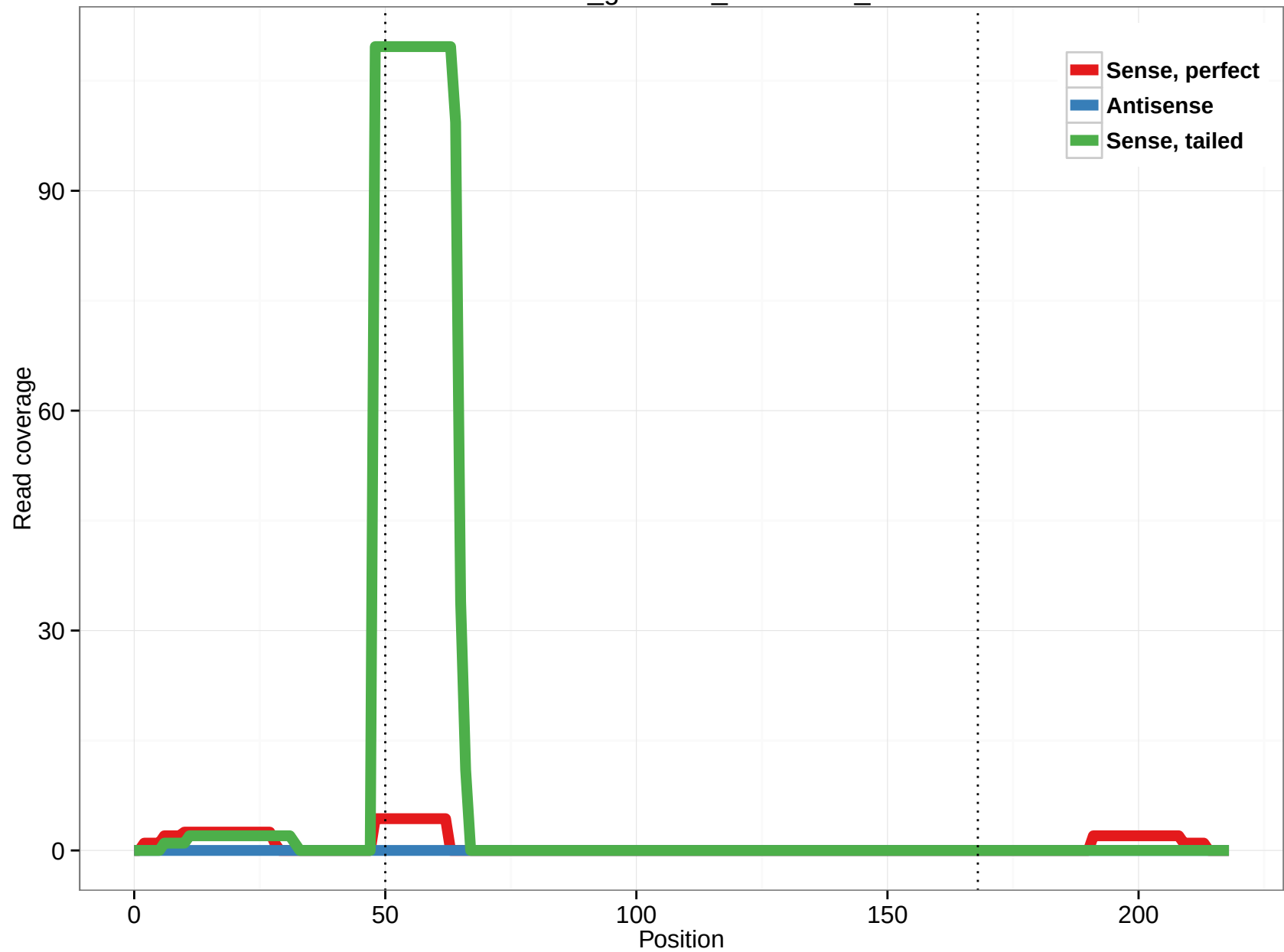
rheMac3_genscan_chr6.2316_9
