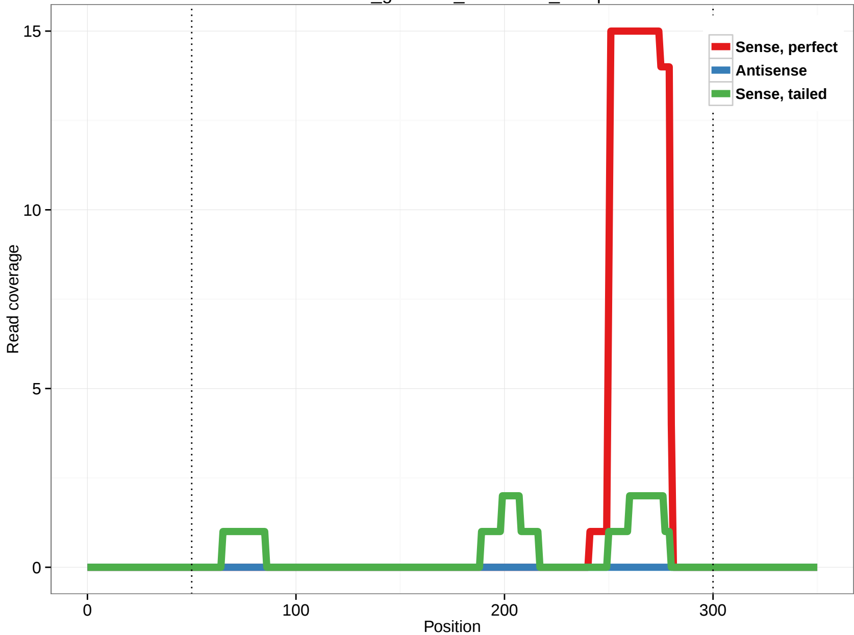
rheMac3_genscan_chr6.2304_11.5p
