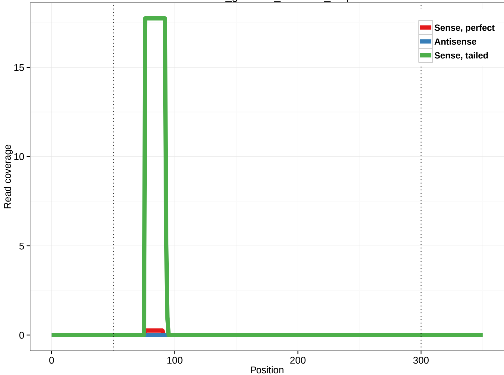
rheMac3_genscan_chr6.227_6.3p
