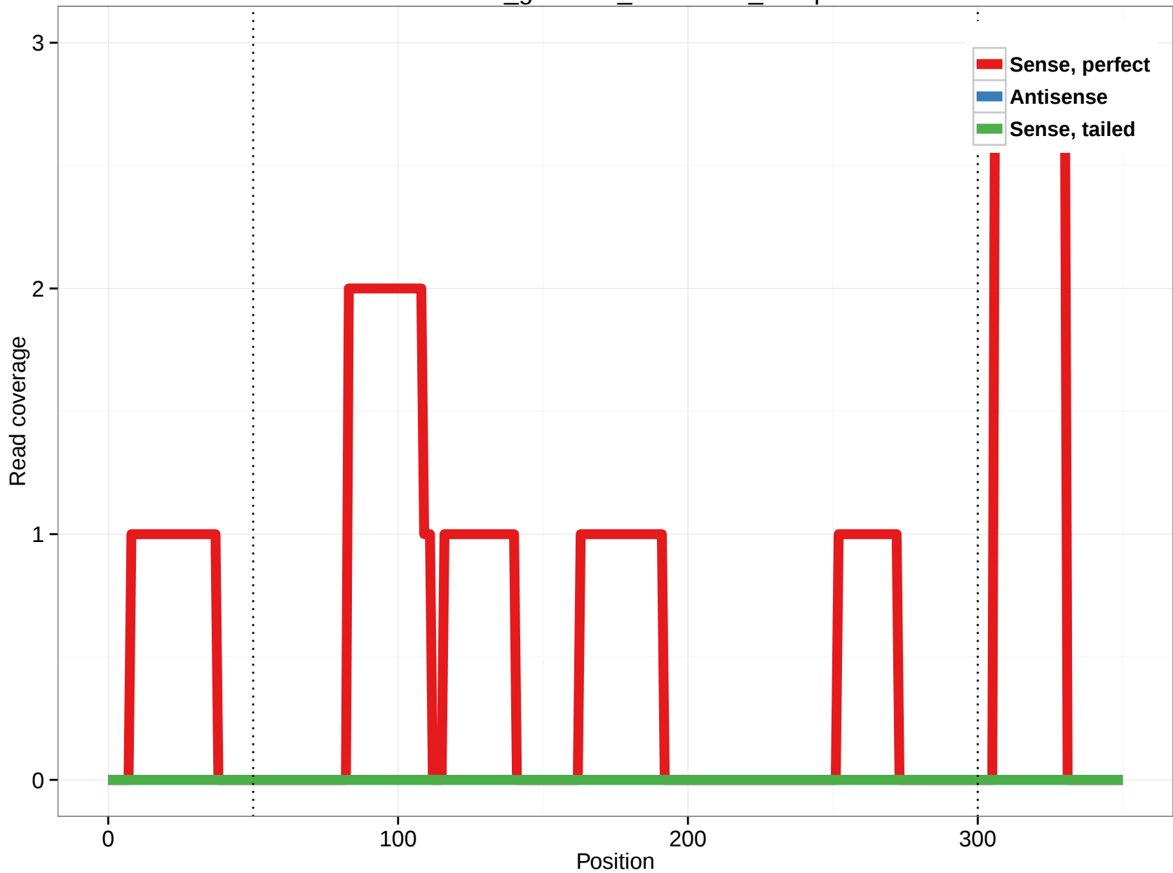
rheMac3_genscan_chr6.2234_18.5p
