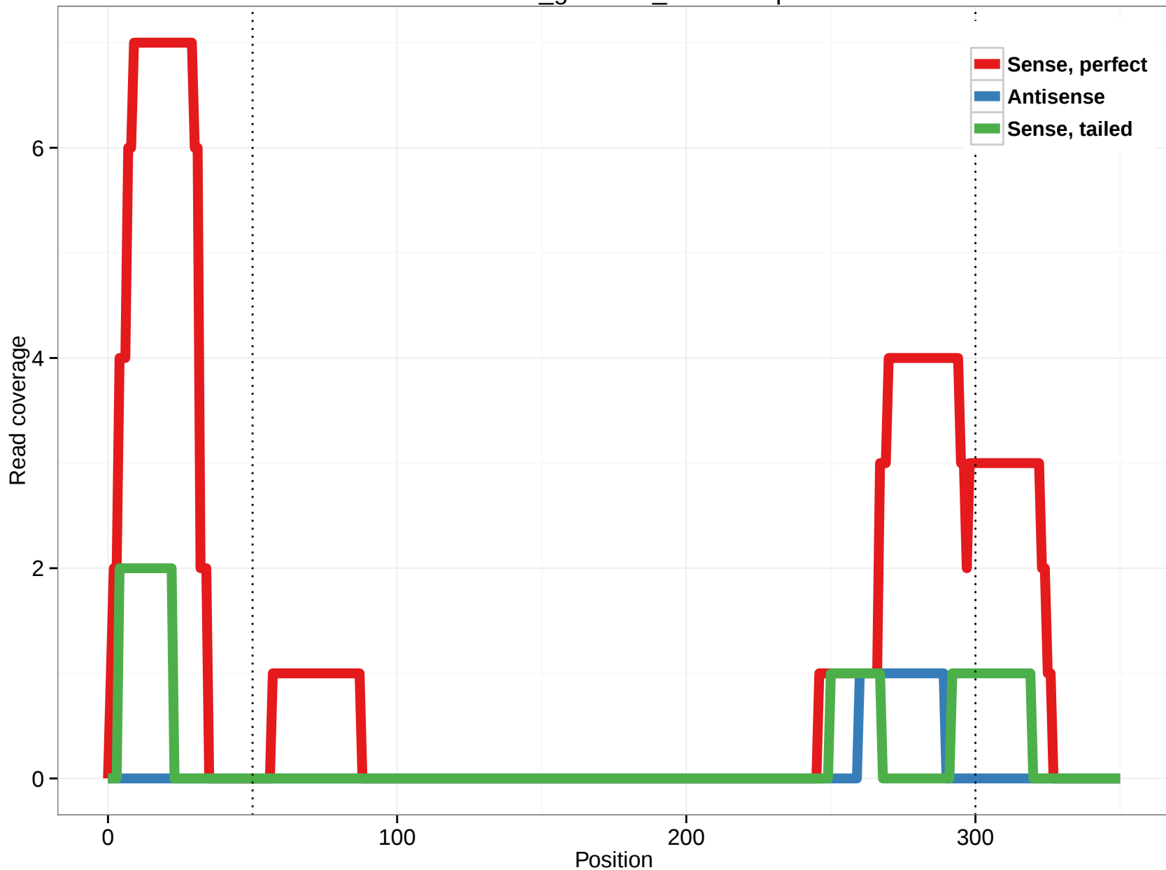
rheMac3_genscan_chr6.22.5p
