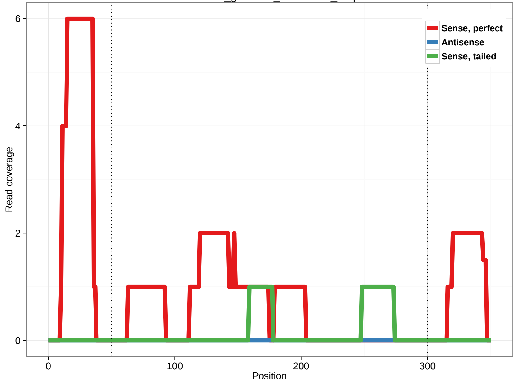
rheMac3_genscan_chr6.2081_1.5p
