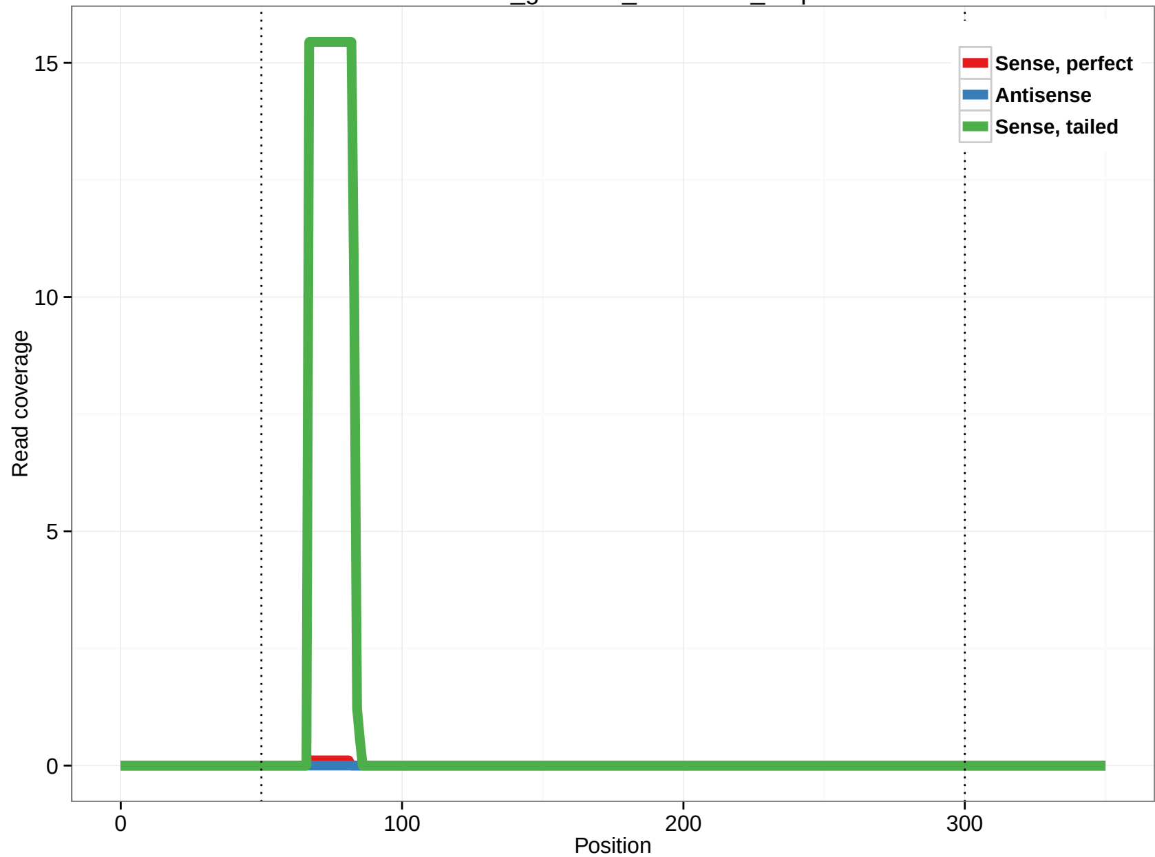
rheMac3_genscan_chr6.1826_6.5p
