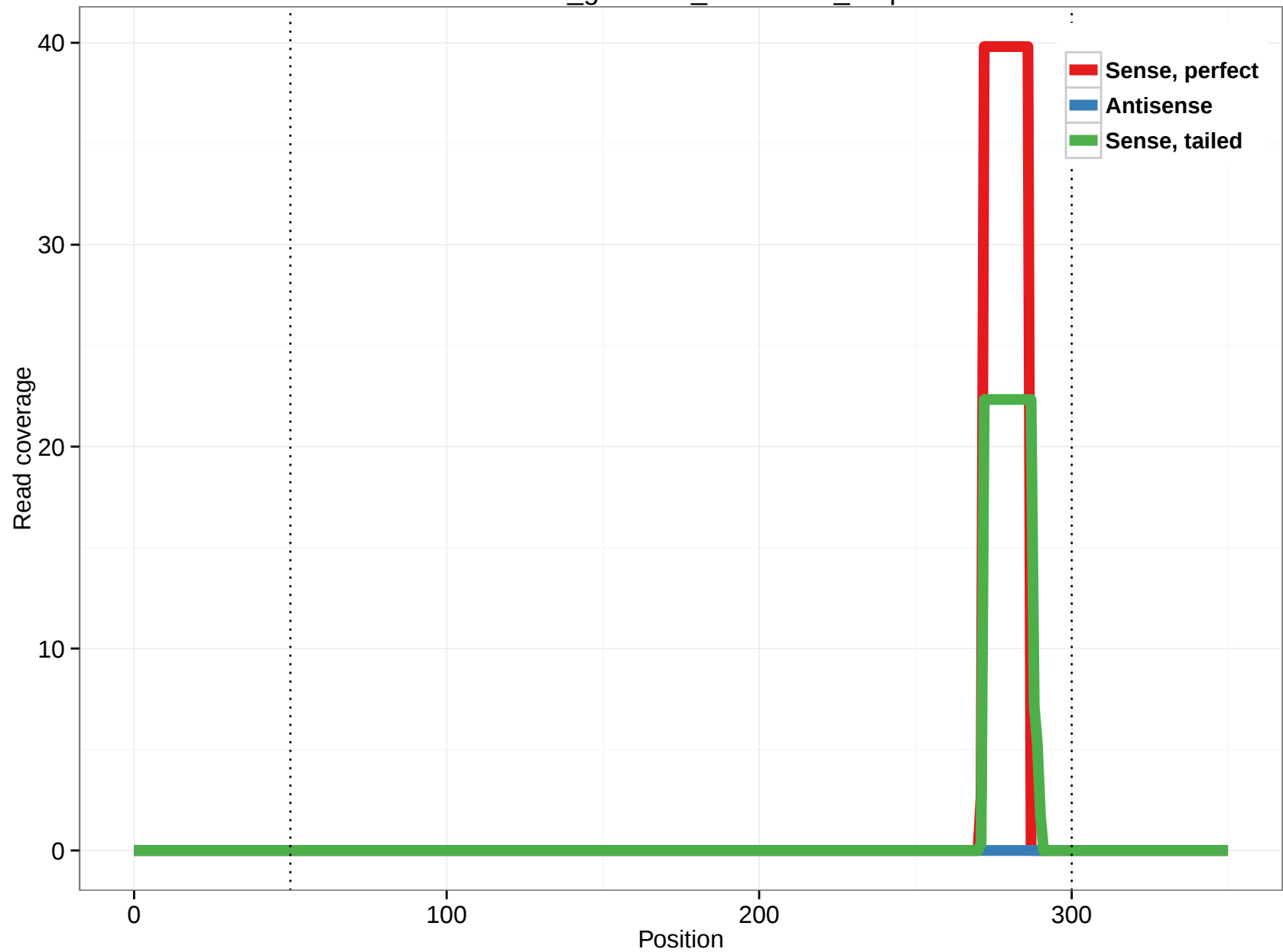
rheMac3_genscan_chr6.1776_4.5p
