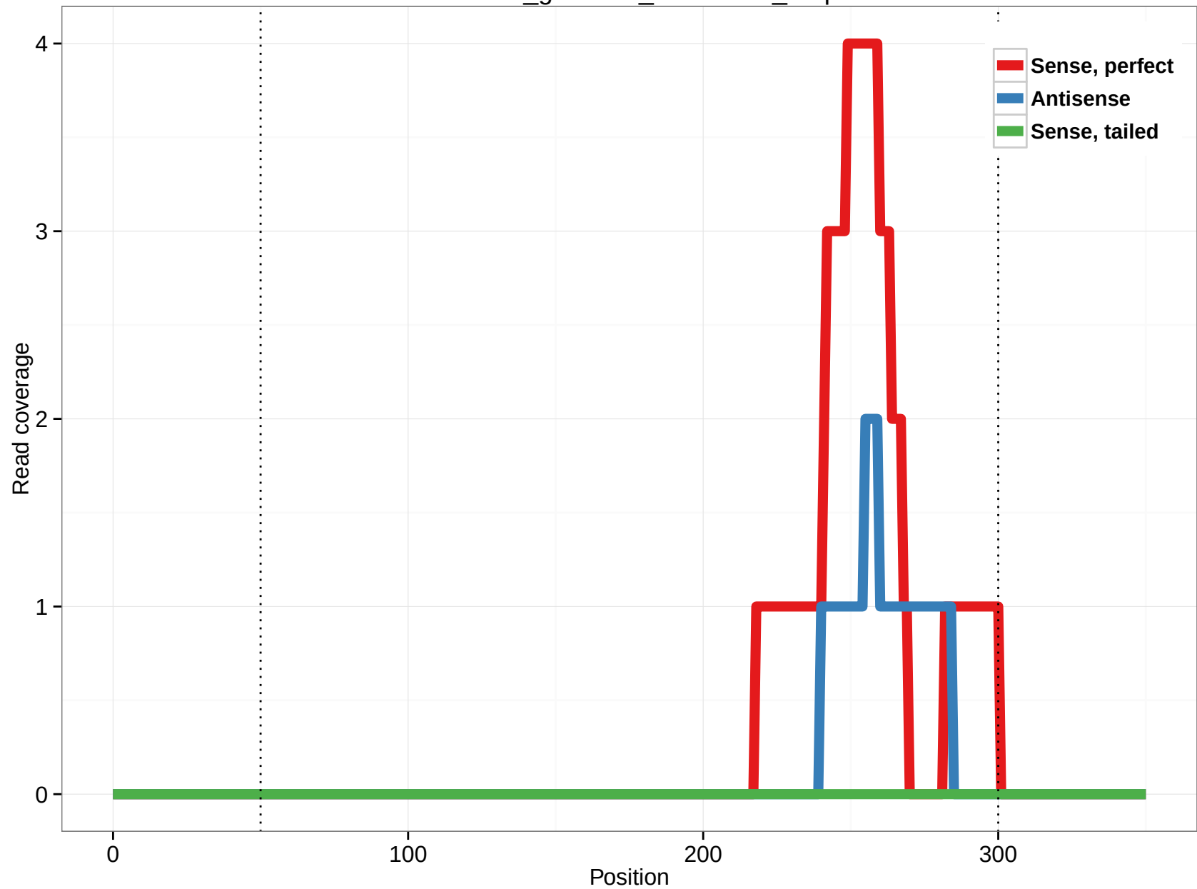
rheMac3_genscan_chr6.1775_0.3p
