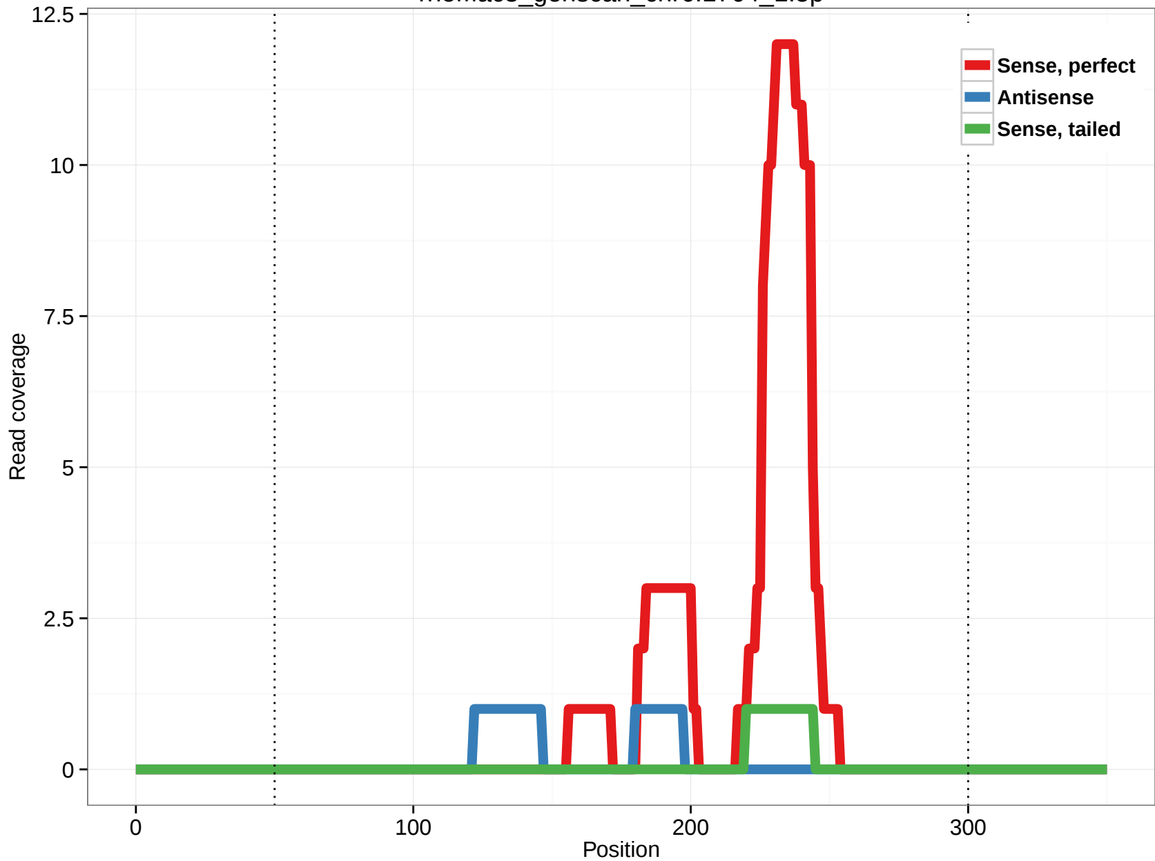
rheMac3_genscan_chr6.1764_1.5p
