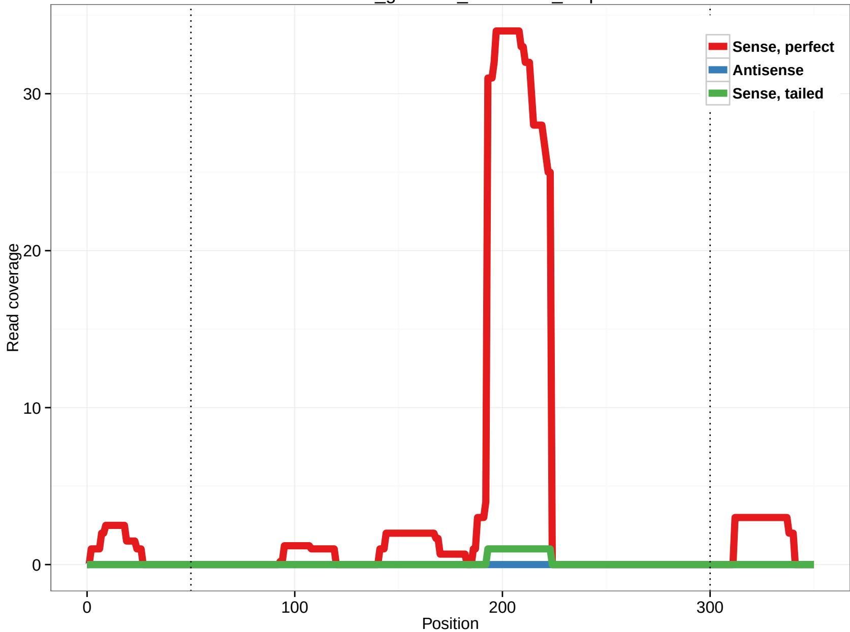
rheMac3_genscan_chr6.1704_5.3p
