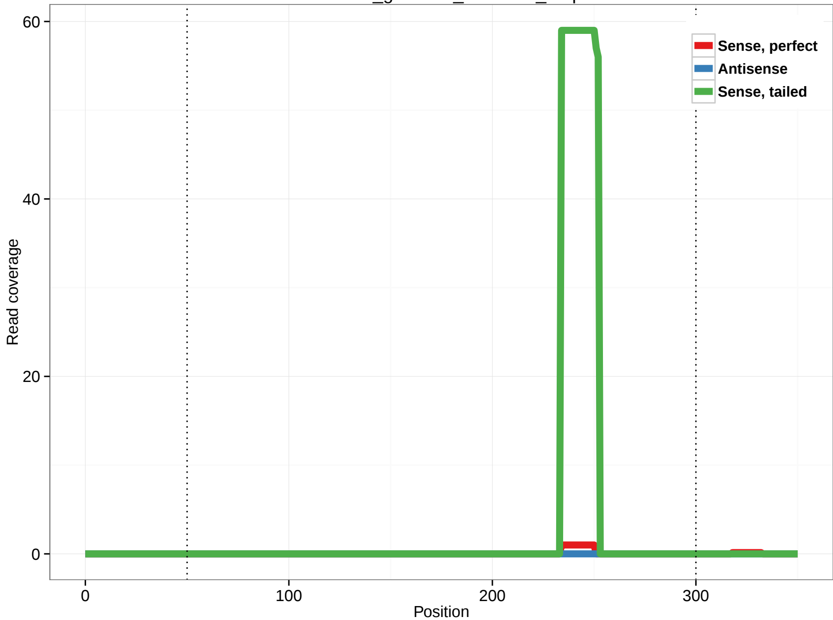
rheMac3_genscan_chr6.168_0.3p
