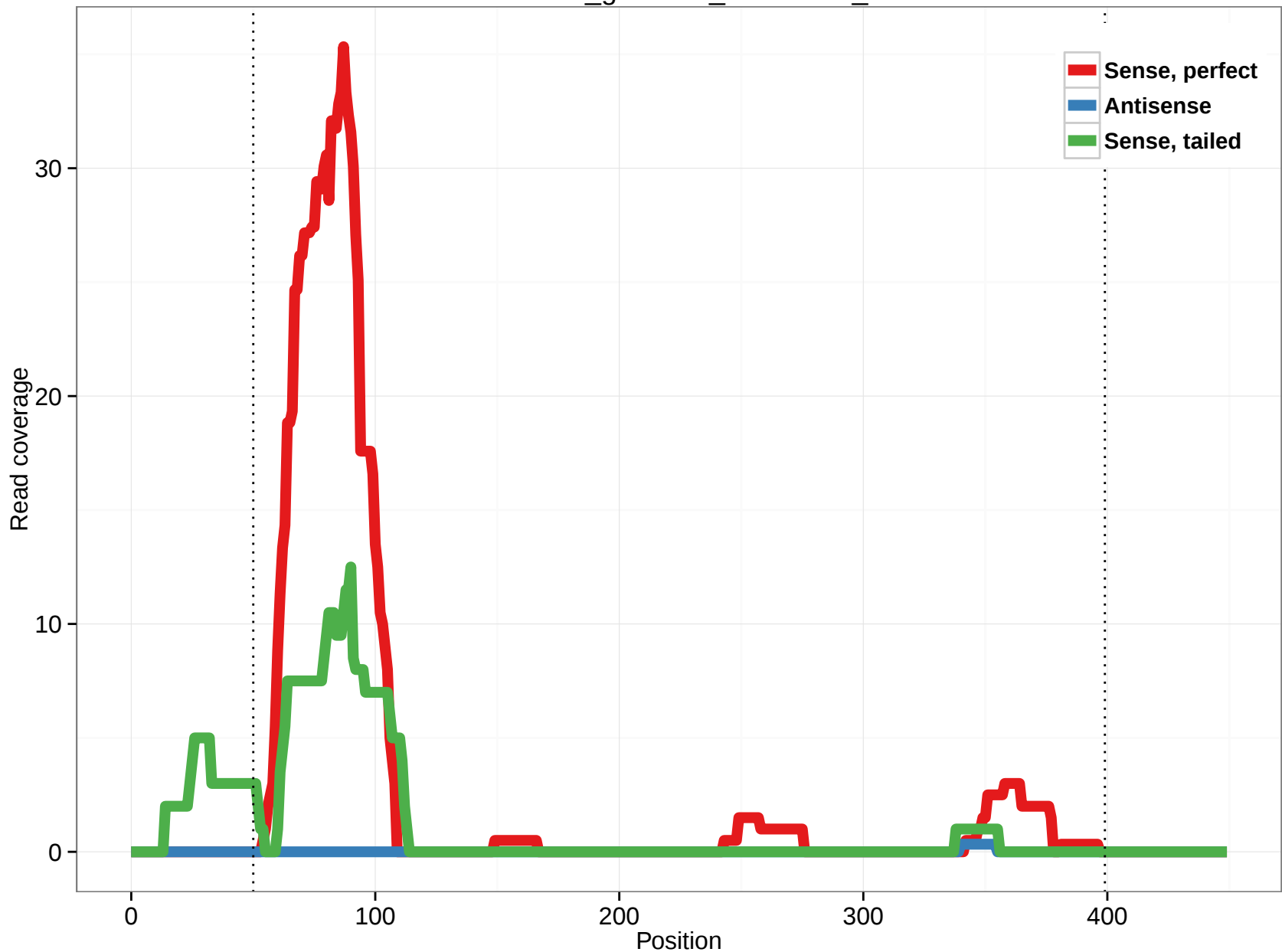
rheMac3_genscan_chr6.1658_0
