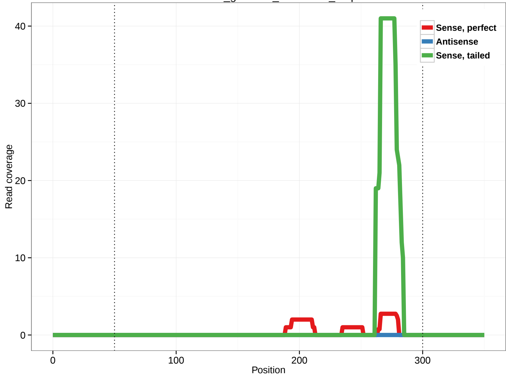
rheMac3_genscan_chr6.1649_0.5p
