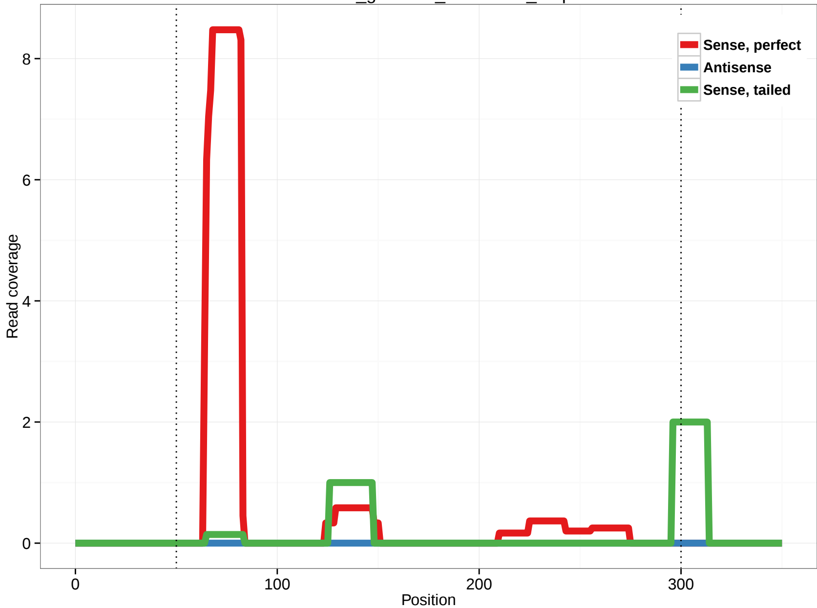
rheMac3_genscan_chr6.1643_8.3p
