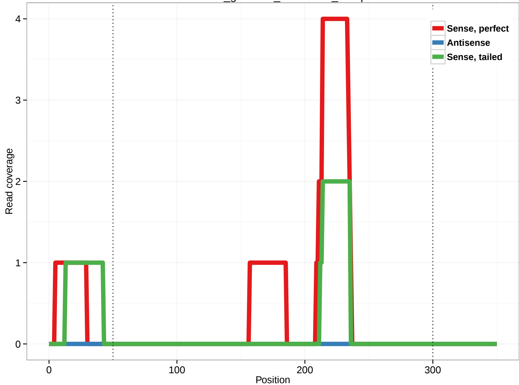
rheMac3_genscan_chr6.1625_10.5p
