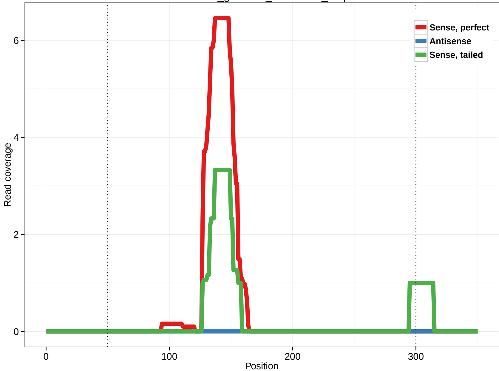
rheMac3_genscan_chr6.1618_2.5p
