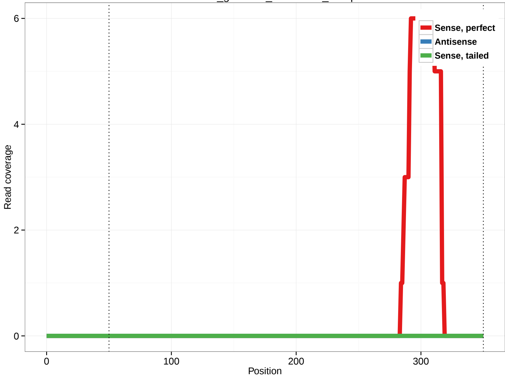
rheMac3_genscan_chr6.1555_20.5p
