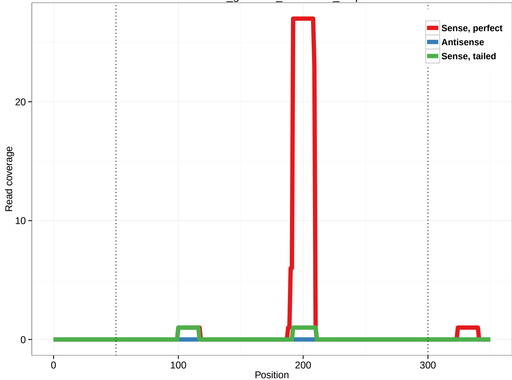
rheMac3_genscan_chr6.1554_1.5p
