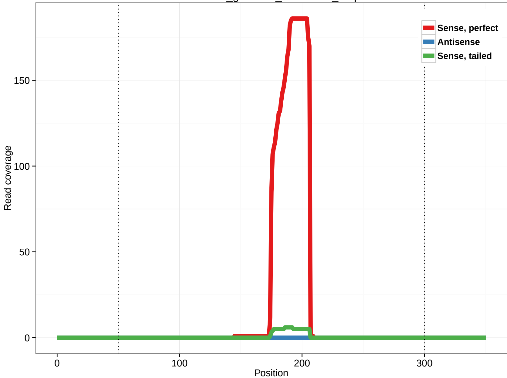
rheMac3_genscan_chr6.1552_4.3p
