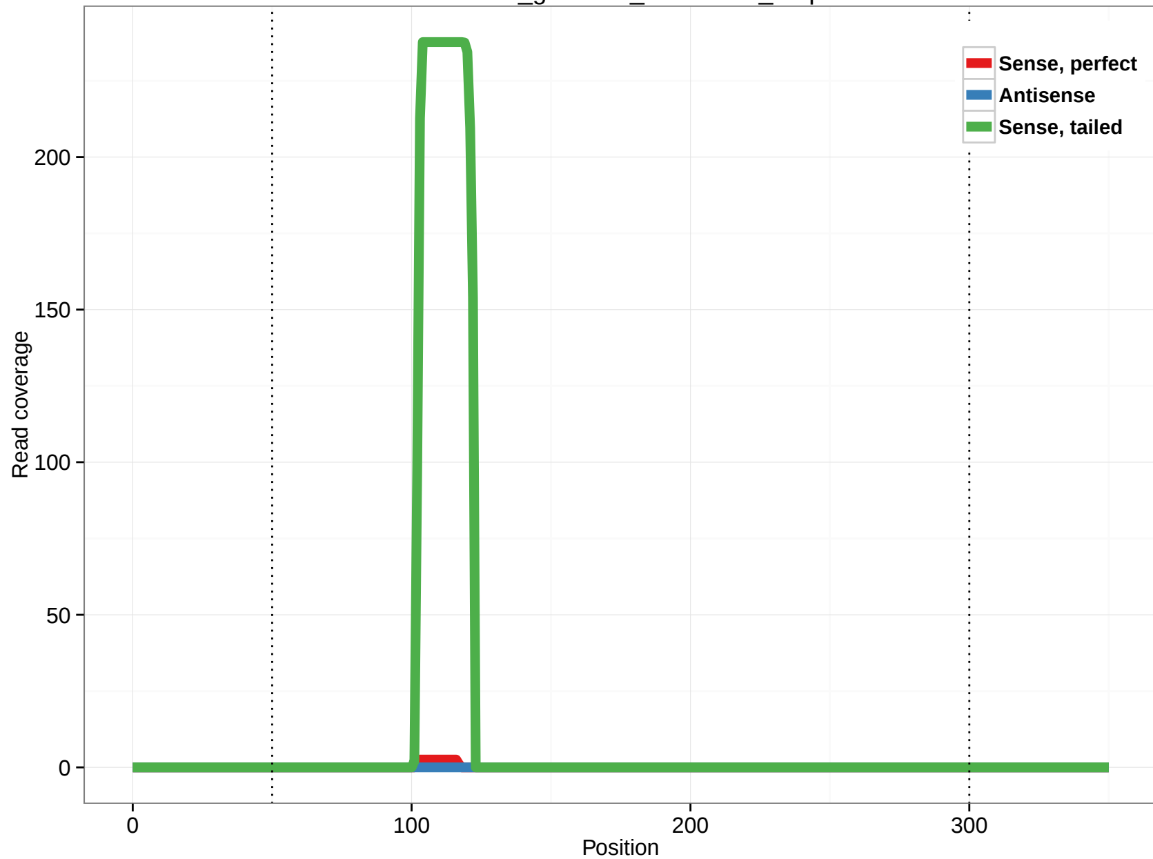
rheMac3_genscan_chr6.1534_0.3p
