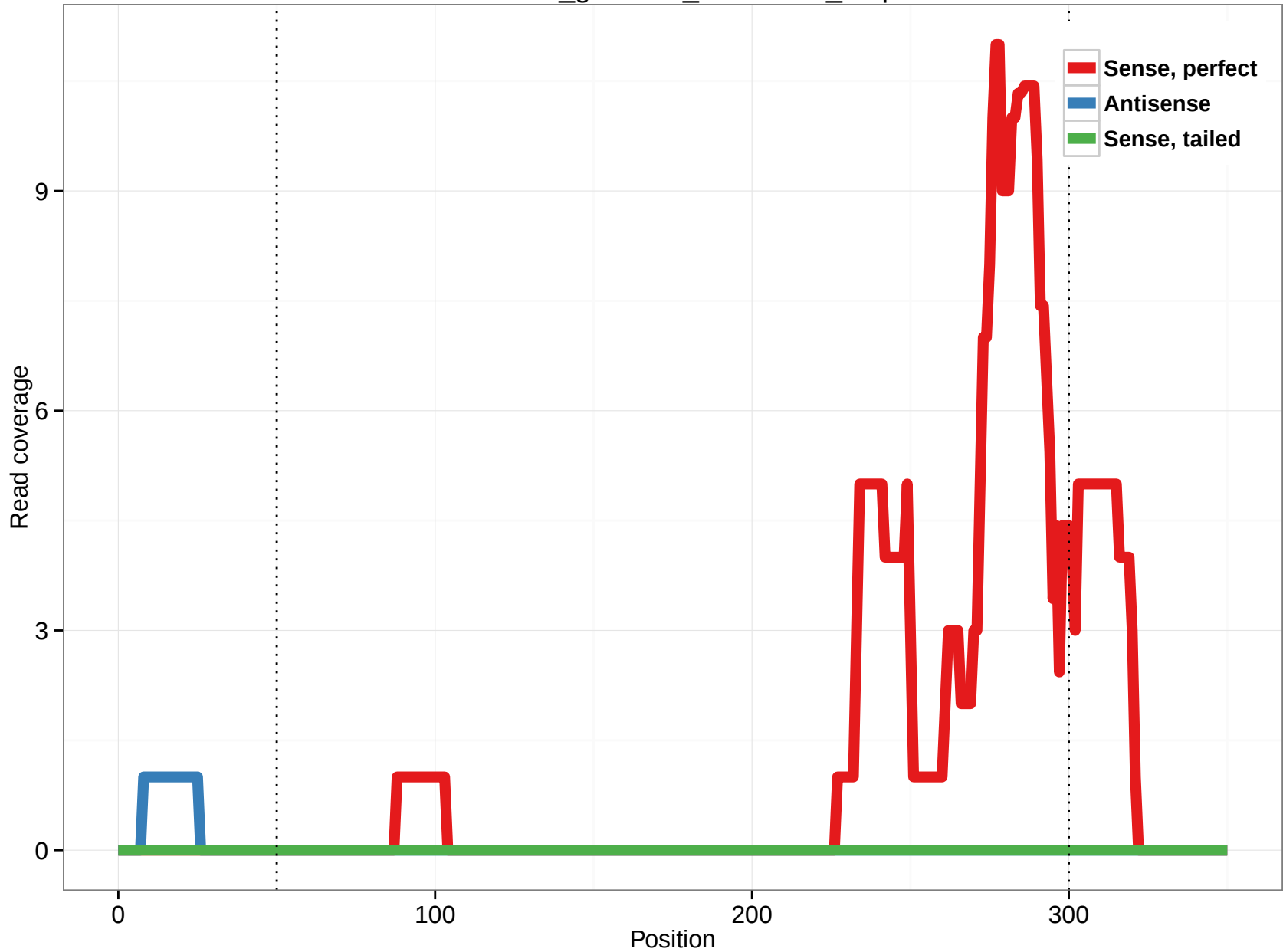
rheMac3_genscan_chr6.1503_1.3p
