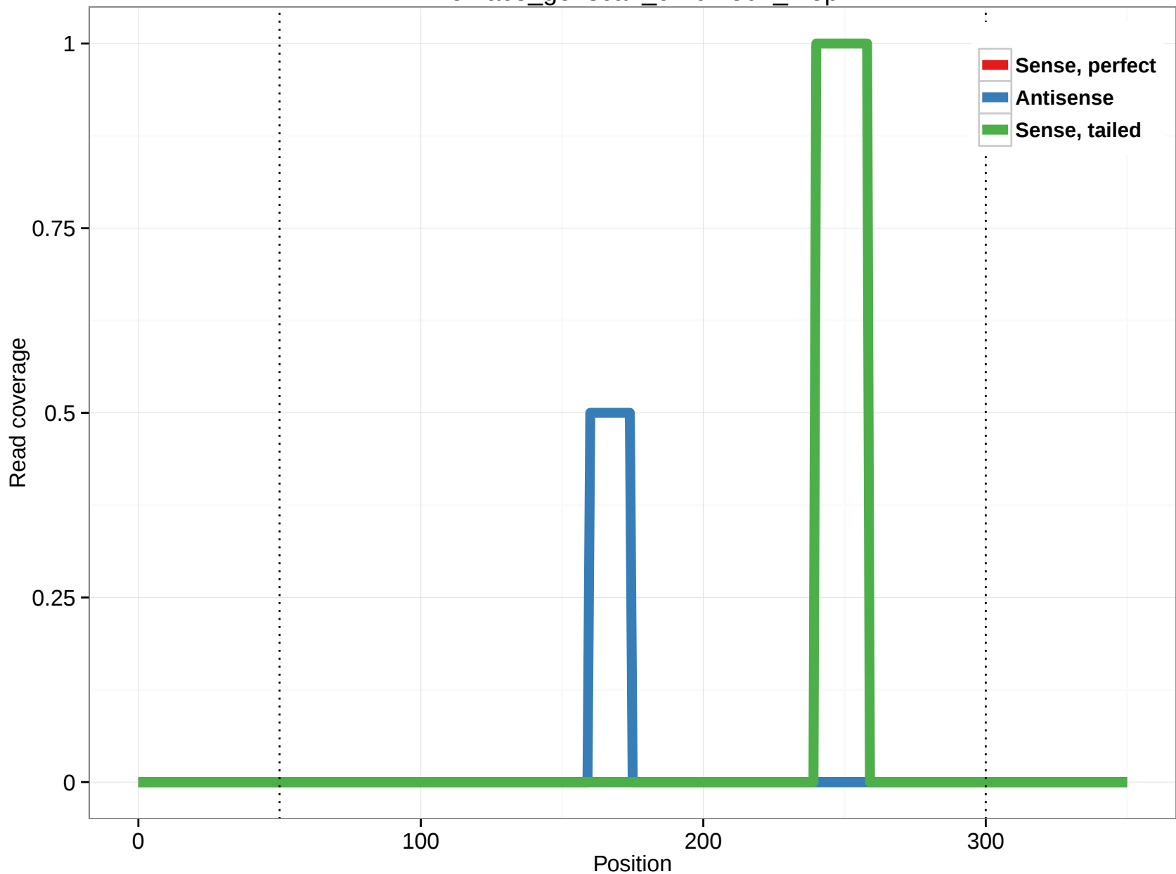
rheMac3_genscan_chr6.1501_1.5p
