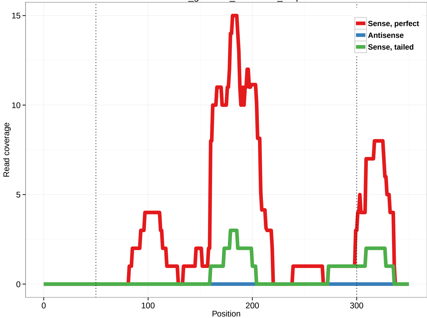
rheMac3_genscan_chr6.1399_6.5p
