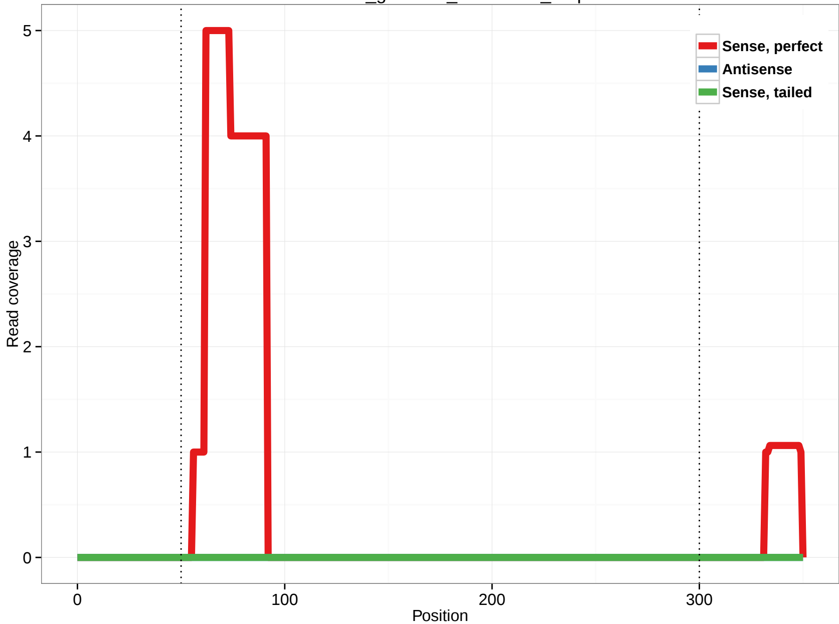
rheMac3_genscan_chr6.1399_6.3p
