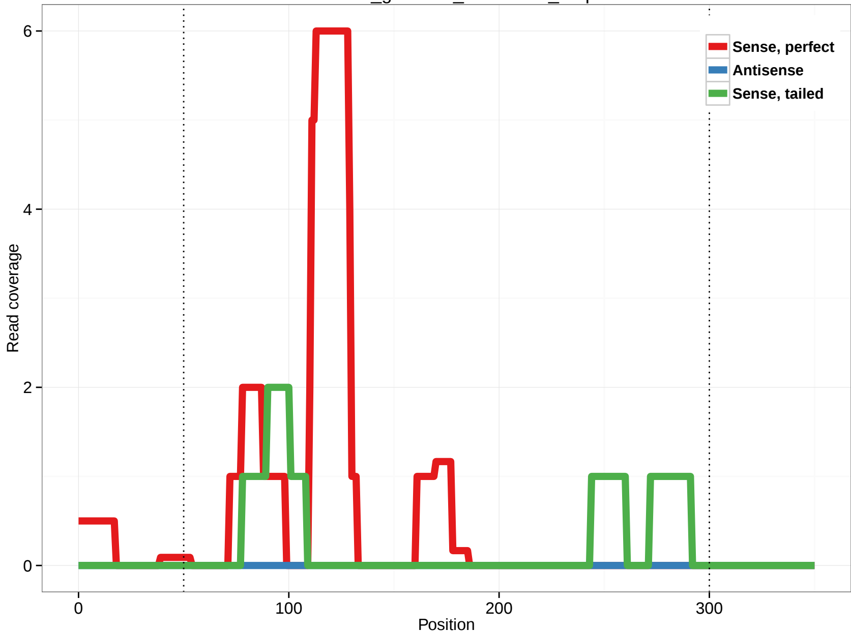
rheMac3_genscan_chr6.1303_1.5p
