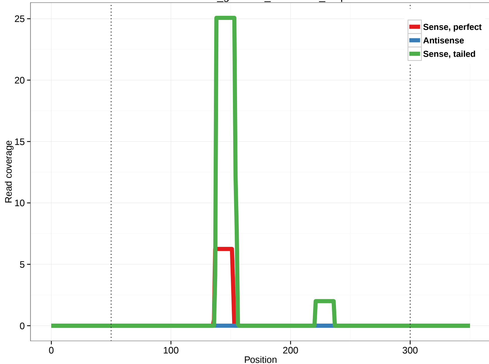
rheMac3_genscan_chr6.1294_2.3p
