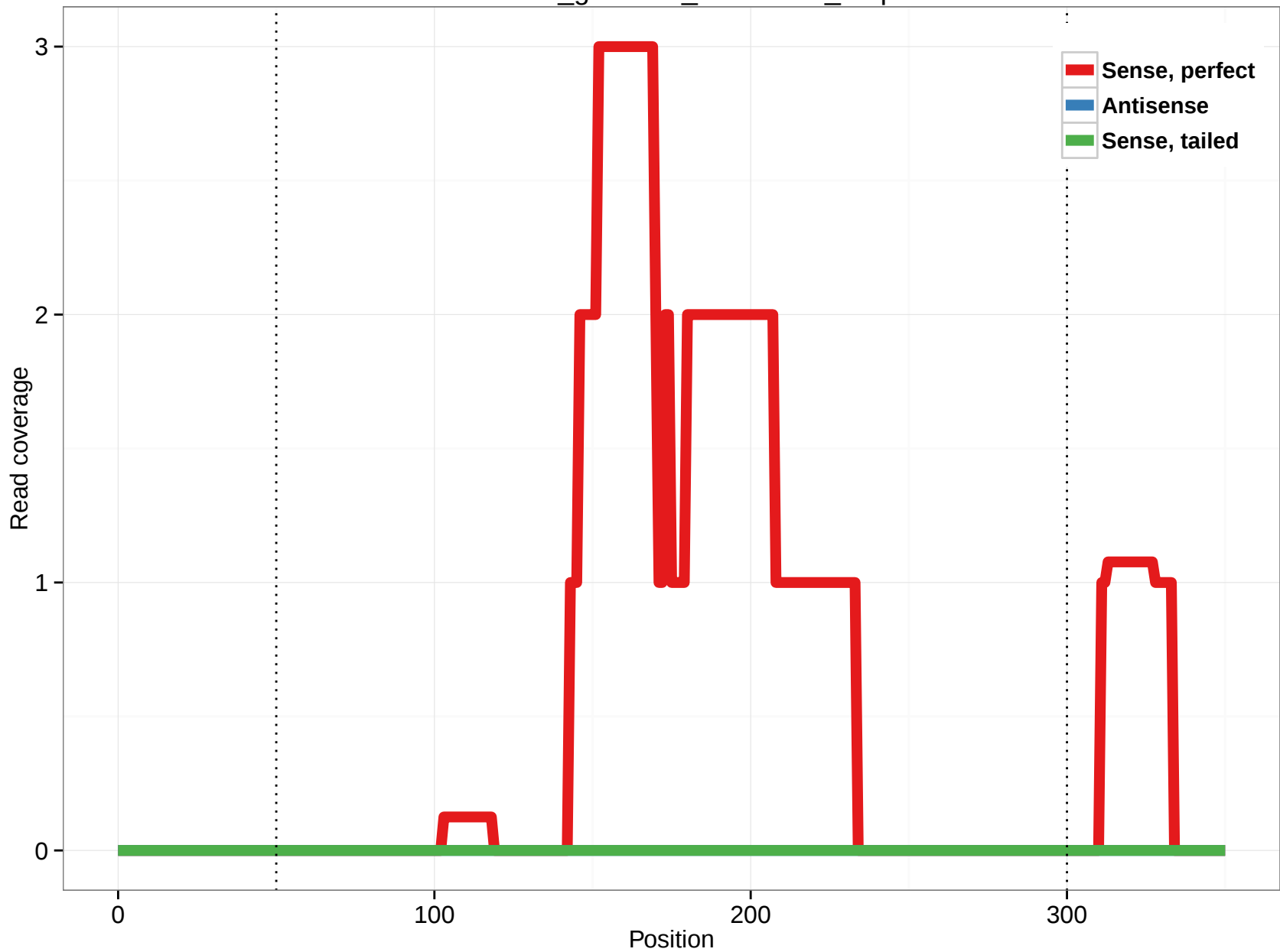
rheMac3_genscan_chr6.1204_3.5p
