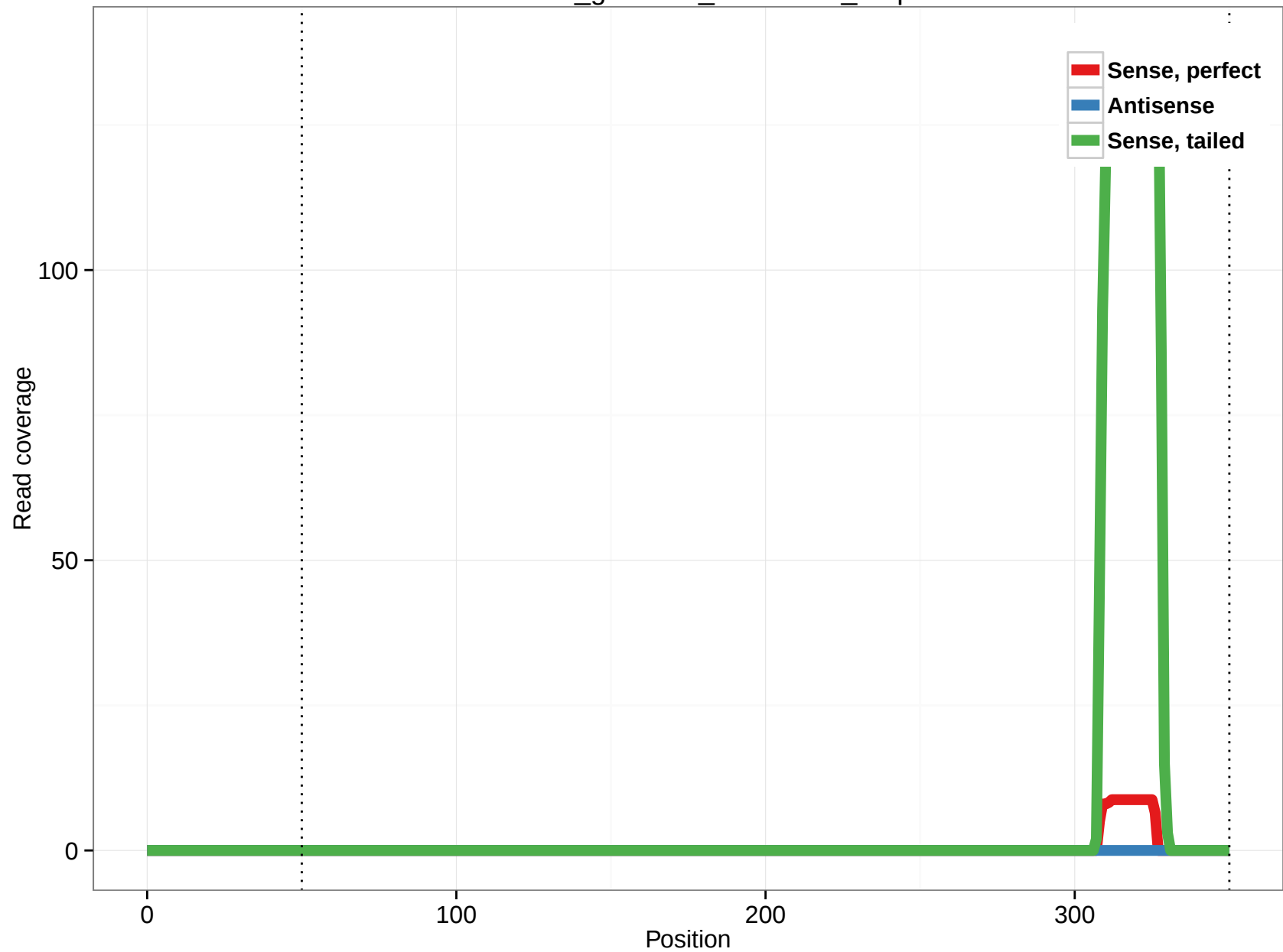
rheMac3_genscan_chr6.1147_0.5p
