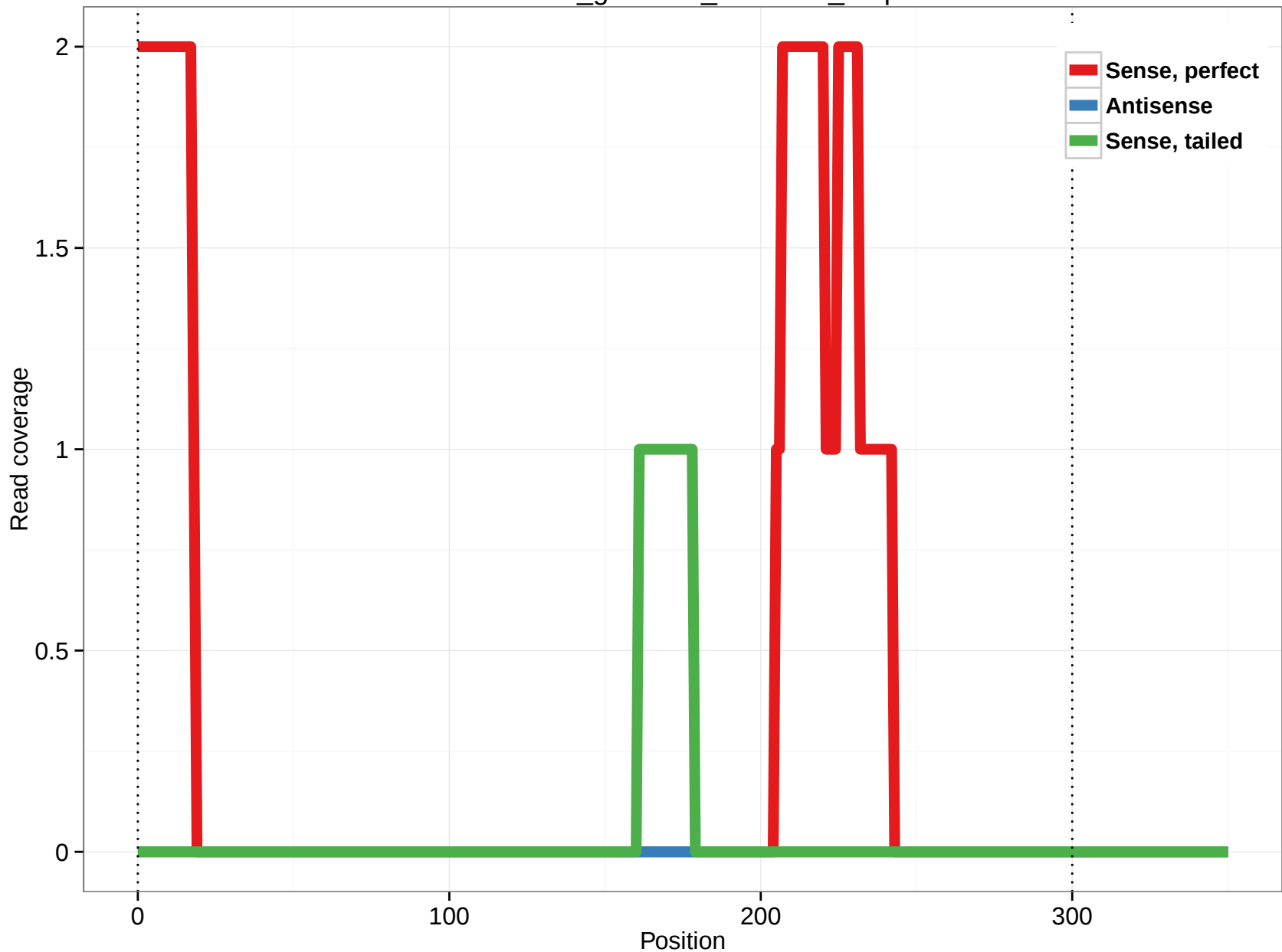
rheMac3_genscan_chr5.715_7.3p
