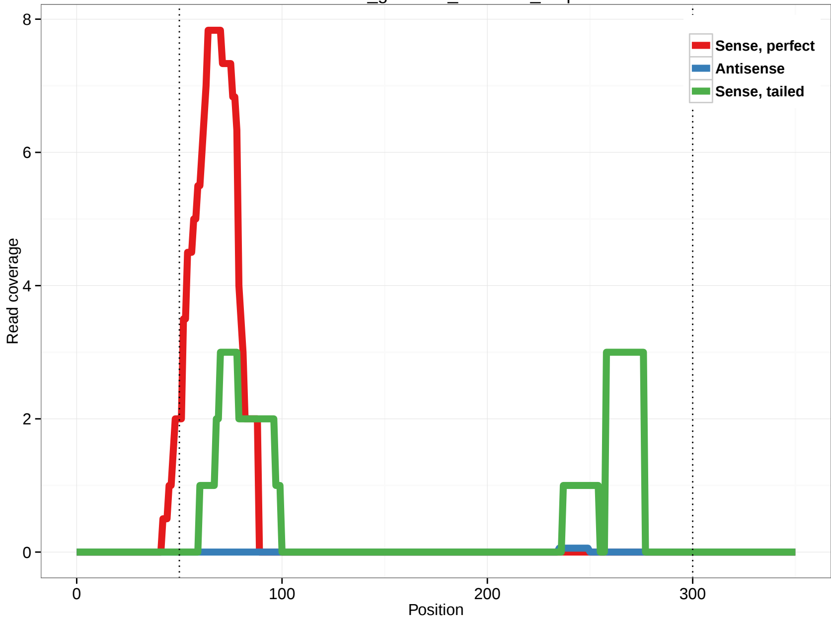
rheMac3_genscan_chr5.620_5.3p
