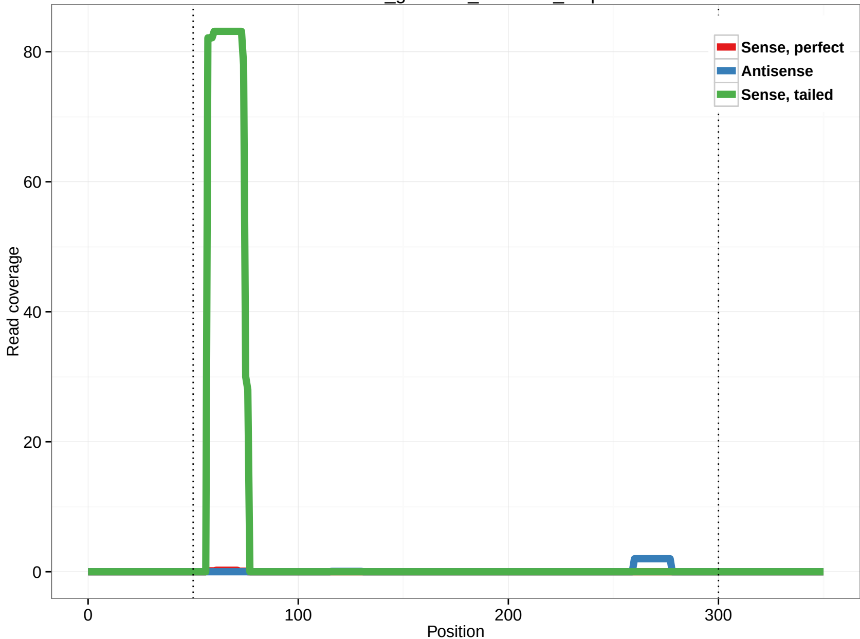
rheMac3_genscan_chr5.399_6.3p
