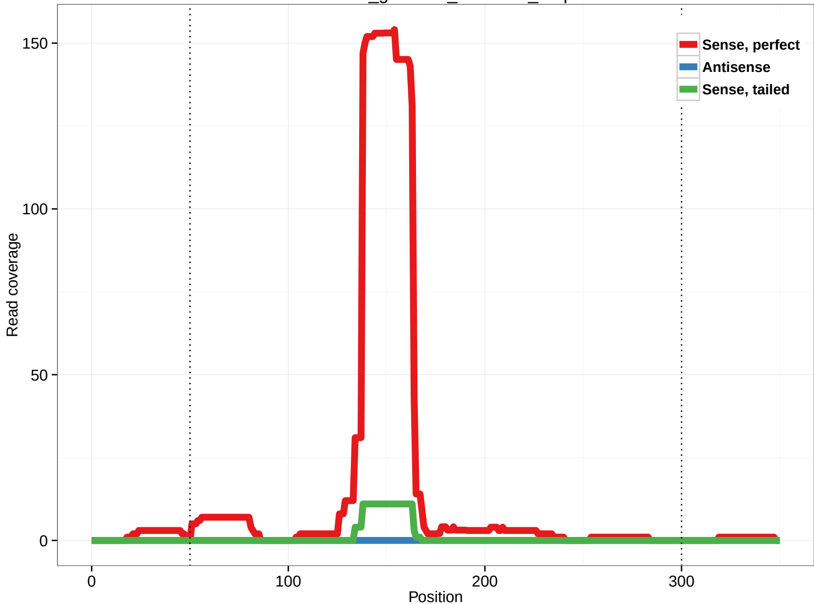
rheMac3_genscan_chr5.393_7.5p
