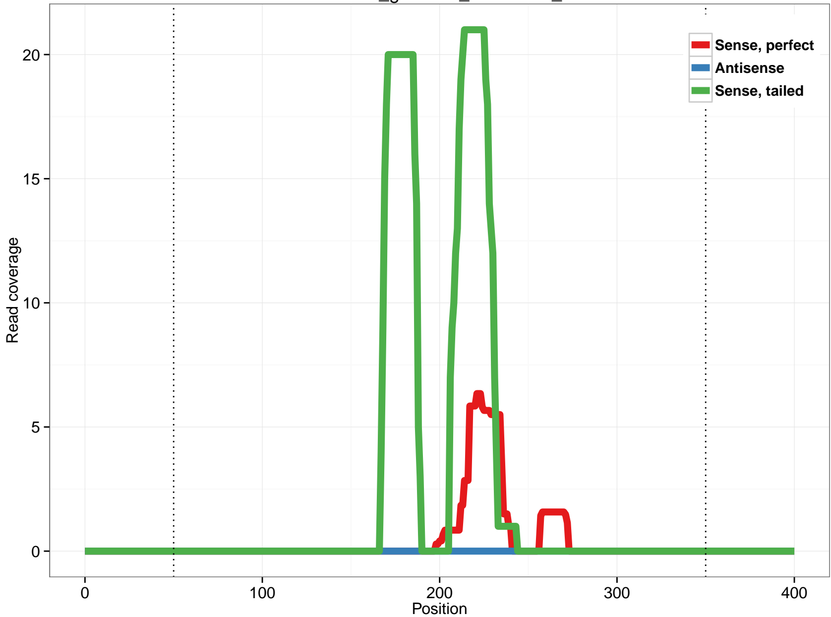
rheMac3_genscan_chr5.2812_3
