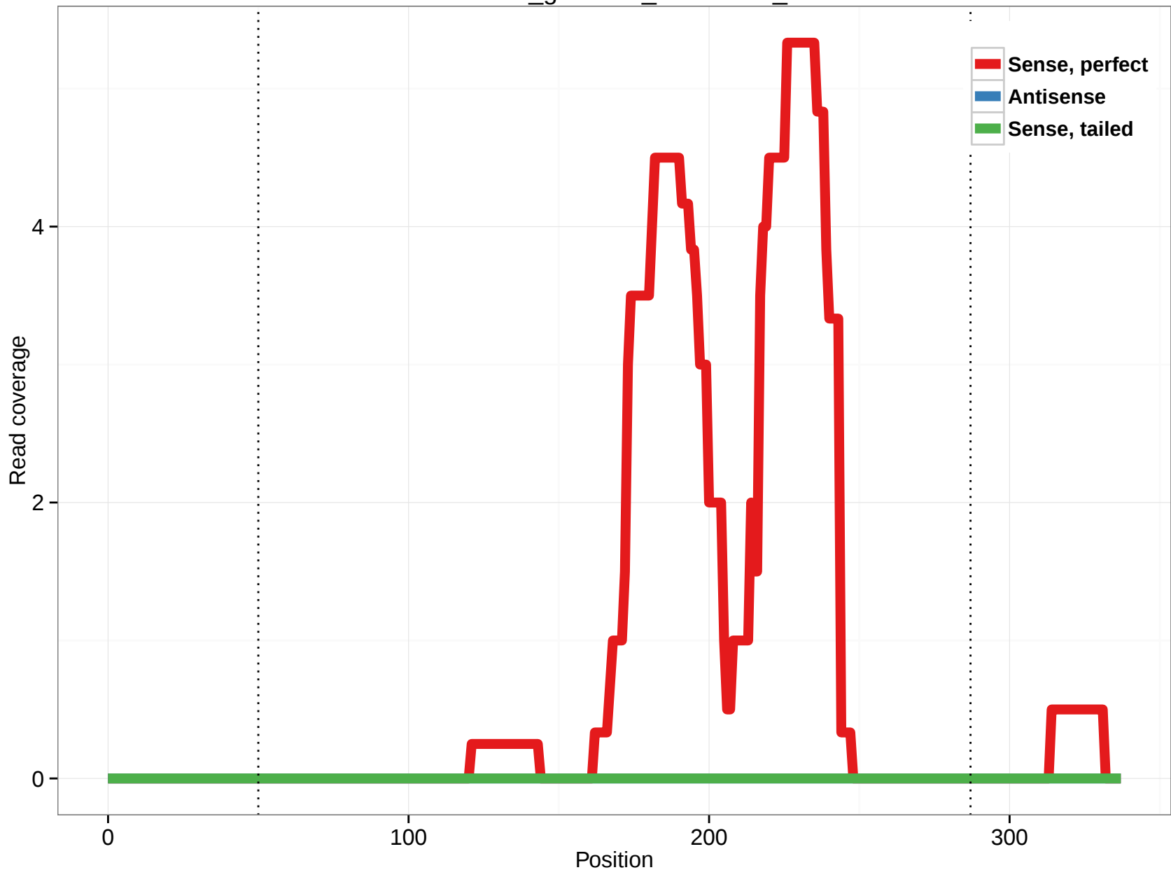
rheMac3_genscan_chr5.2798_0
