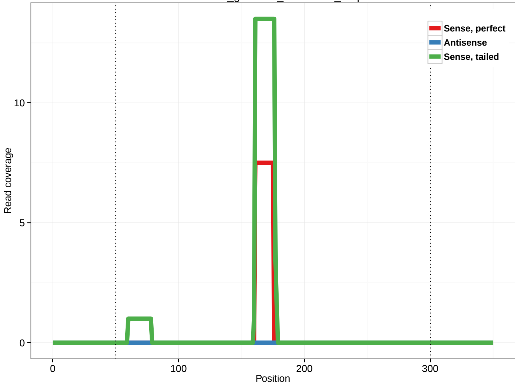
rheMac3_genscan_chr5.2682_1.3p
