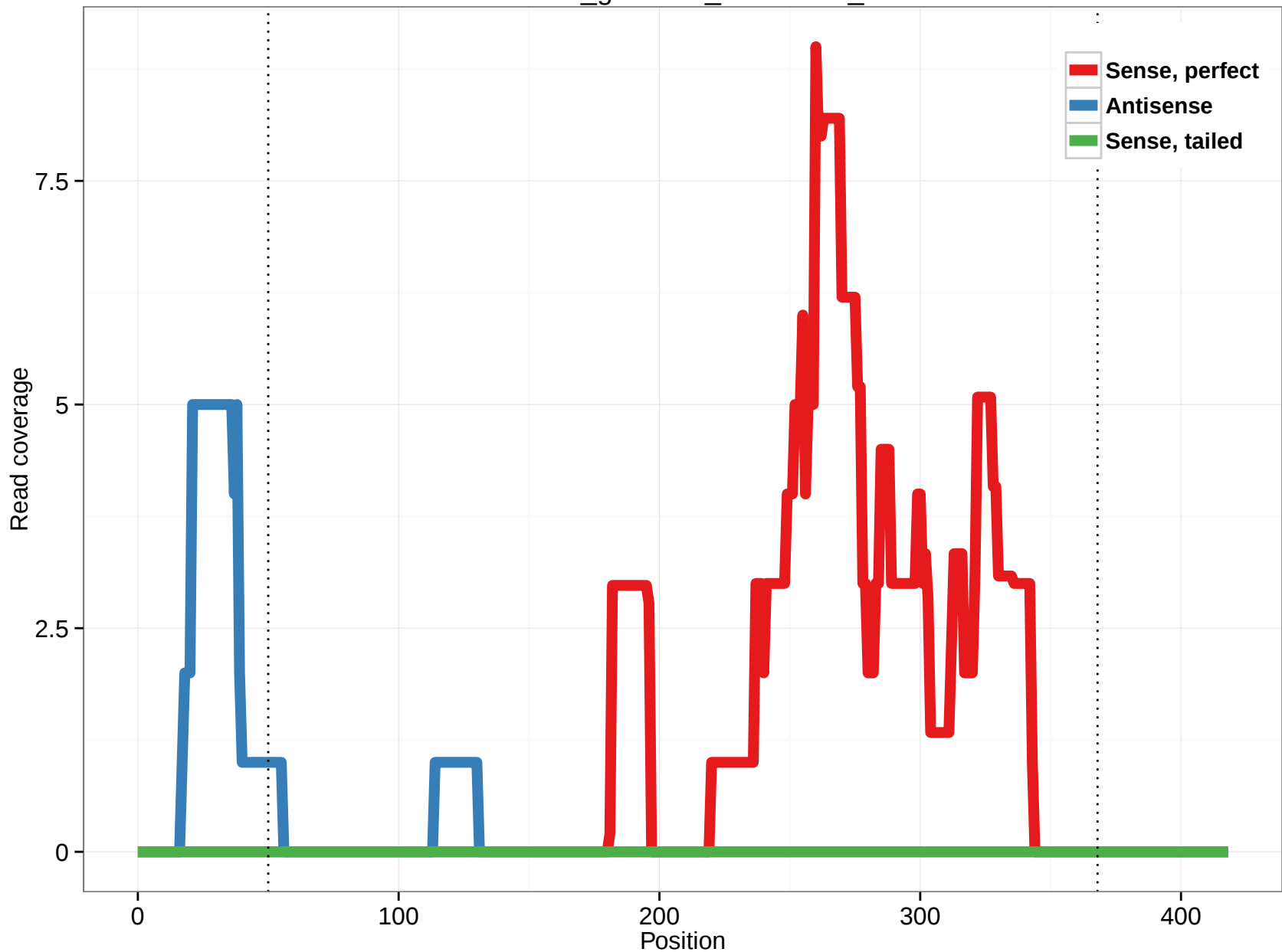
rheMac3_genscan_chr5.2596_11
