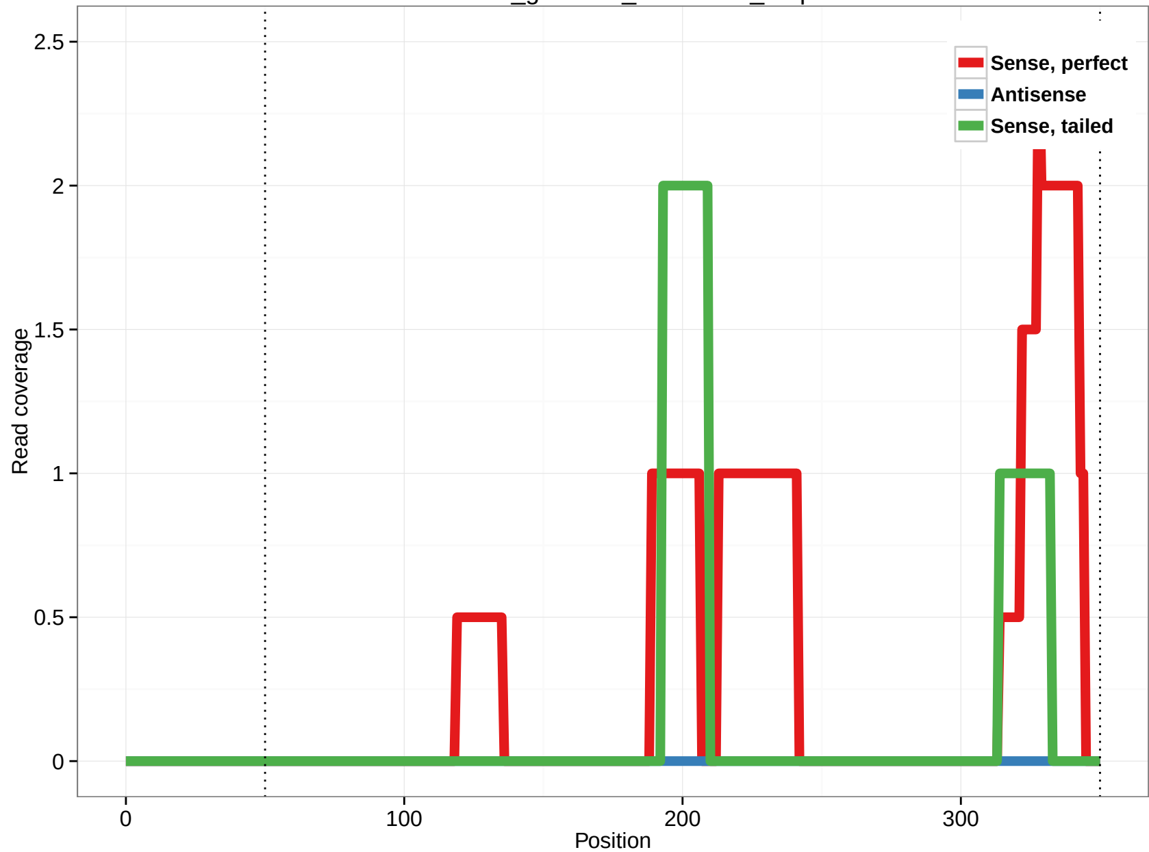
rheMac3_genscan_chr5.2435_1.5p
