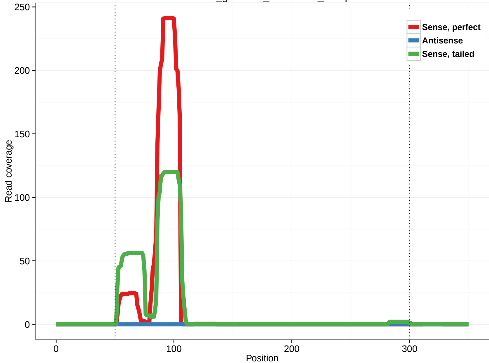
rheMac3_genscan_chr5.2321_20.5p
