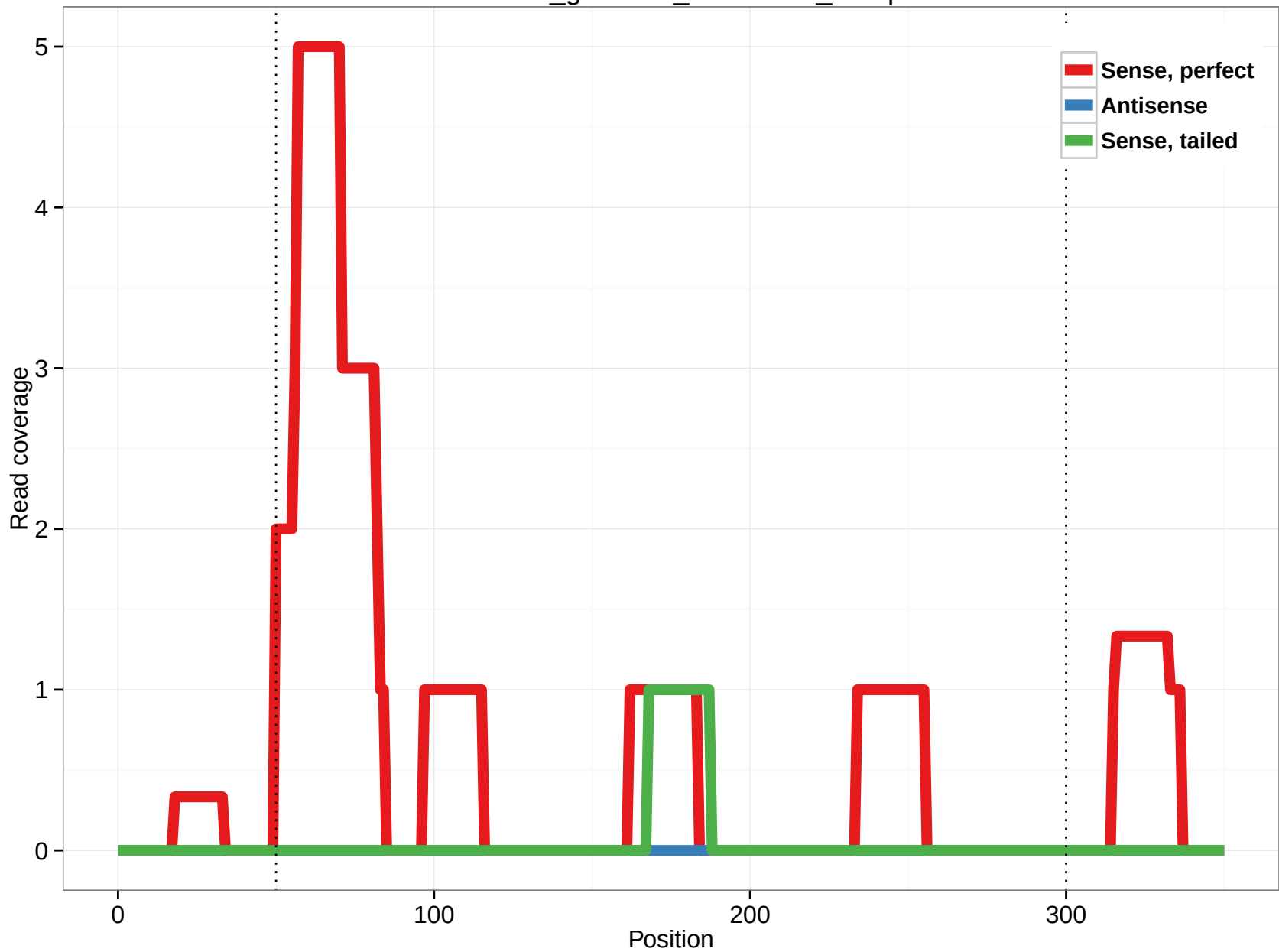
rheMac3_genscan_chr5.2309_13.5p
